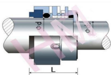
HMFR-02-E(Vulcan Y-XX08/2)
